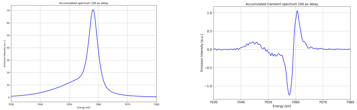
Figure 7: On the left the XES spectrum with the excitation laser on at a delay of 100 ps is plotted. On the right there's the difference spectrum at the same time delay.
