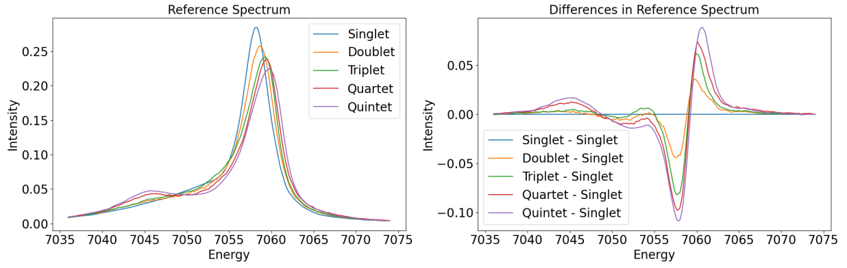
Figure 6: The reference spectra plotted with provided data for different spin states. The reference difference spectra with transient signals plotted with provided data for different transitions.
