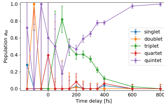
Figure 8: The population curves of the different spin states plotted against the time delay of the optical laser in femtoseconds.
